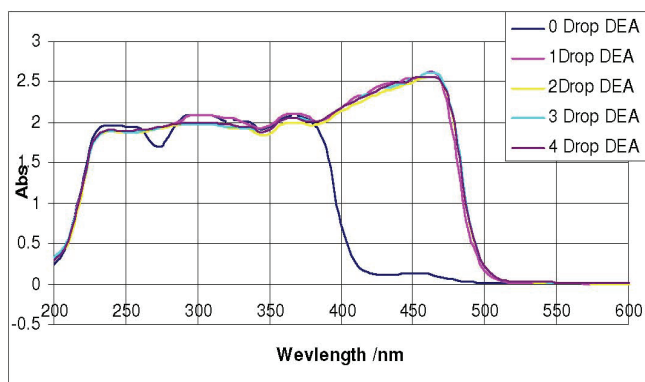
Fig. 2. UV – visible spectra of vanillin 2 in ethanol at various amounts of DEA.
