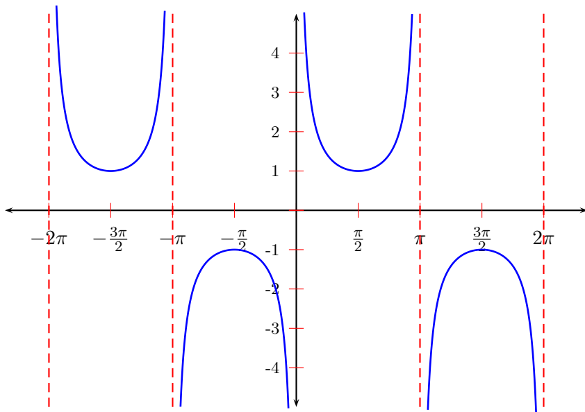
The graph of y = \csc x
