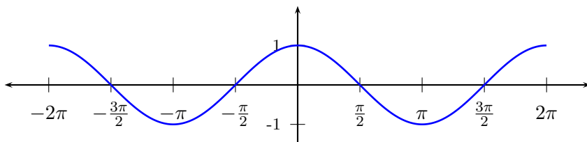
The graph of y = \cos x
