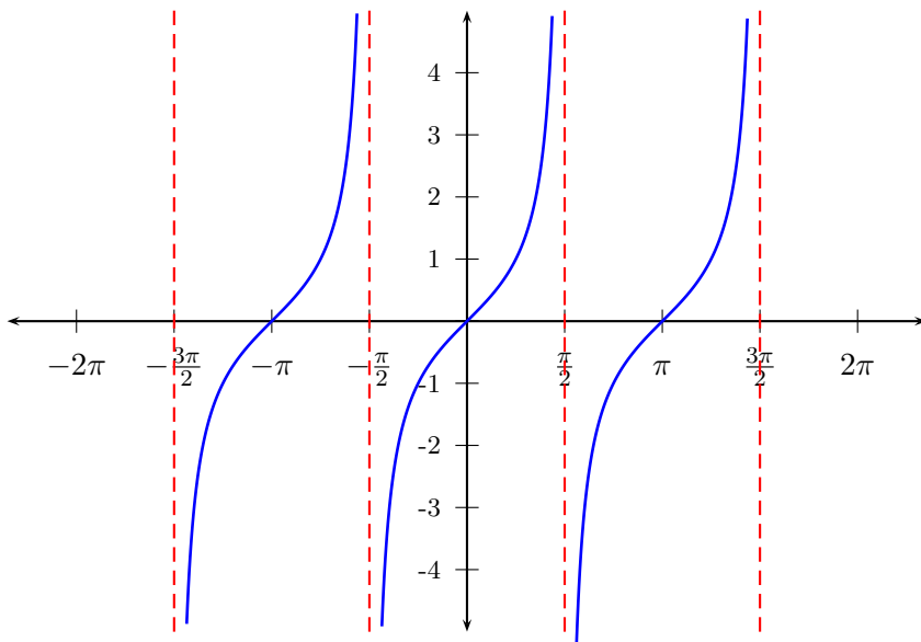
The graph of y = \tan x
