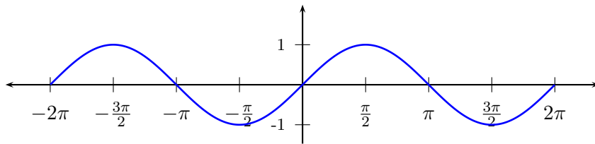
The graph of y = \sin x
