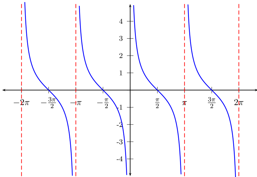
The graph of y = \cot x
