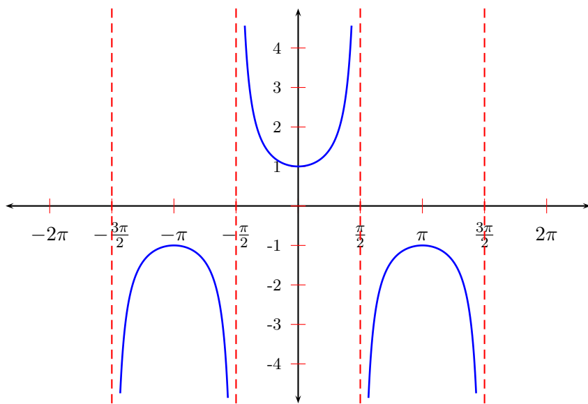
The graph of y = \sec x
