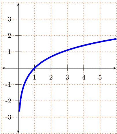
The graph of y = \ln x
