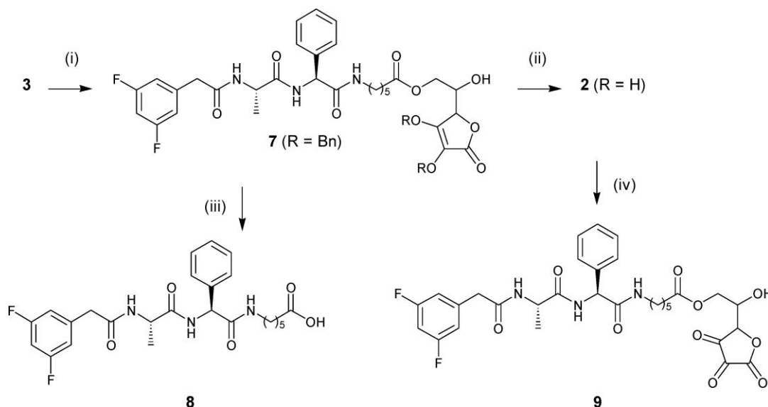
Scheme 3 Conditions and reagents: (i) 6 , BOP, DIEA, CH 2 Cl 2 , rt; 73%; (ii) H 2 , Pd(OH) 2 /C, MeOH, rt; 90%; (iii) LiOH, CaCl 2 , iPrOH–H 2 O (v/v, 7 : 3), rt; 58%; (iv) H 2 O 2 , MeOH, rt.
